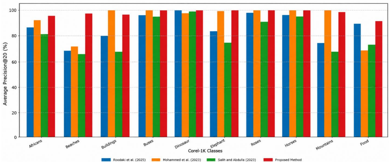
Figure 6. Class-wise average precision (%) comparison of the proposed method with existing CBIR methods on the Corel-1K dataset.
