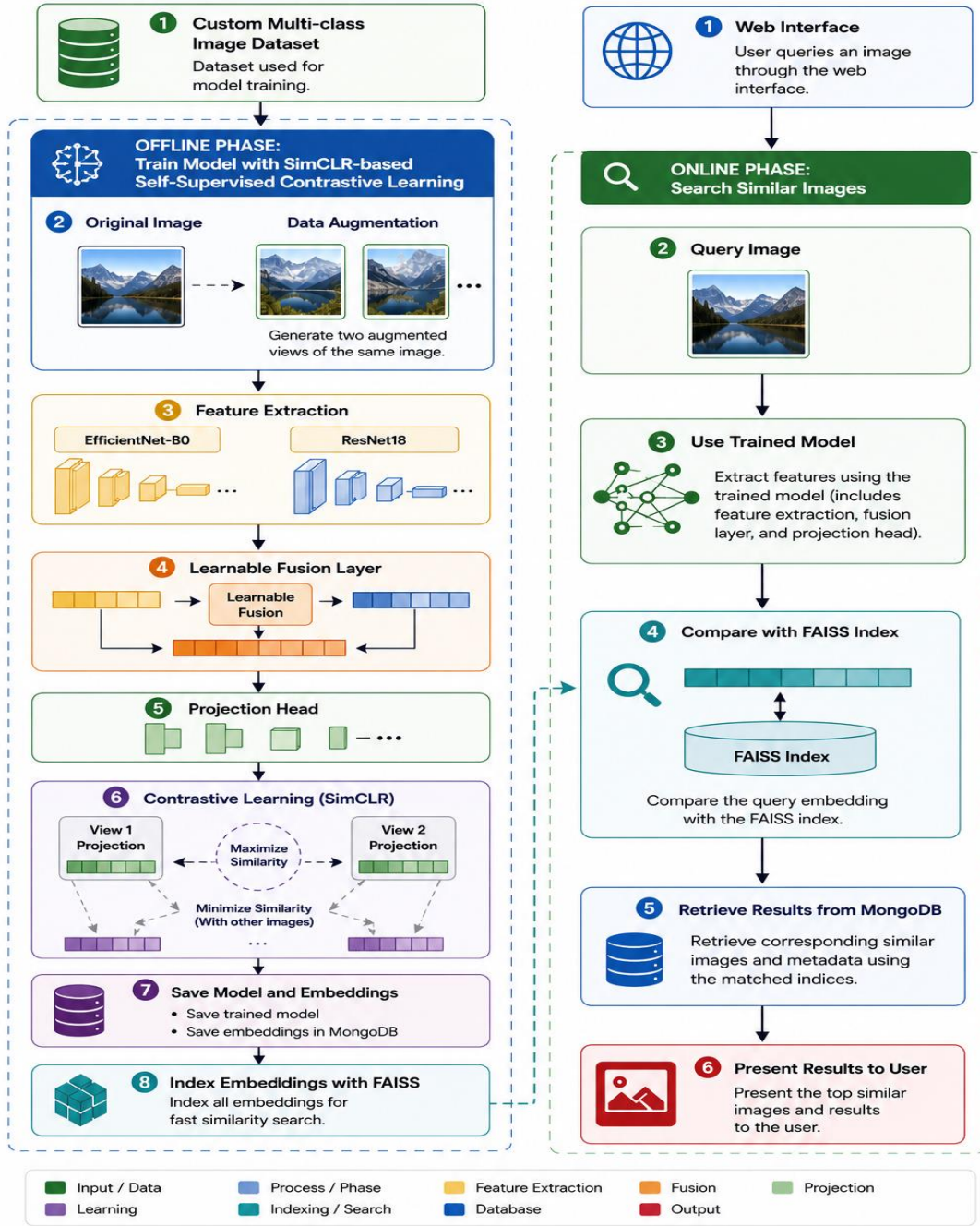
Figure 1. Overall architecture of the proposed CBIR system showing the complete pipeline from hybrid feature extraction to similarity-based image retrieval in a unified framework.
