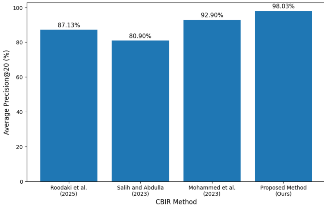
Figure 7. Comparison of Average Precision@20 (%) between the proposed method and literature-reported CBIR methods on the Corel-1K dataset.
