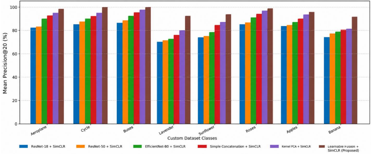
Figure 5. Class-wise Mean Precision@20 comparison of different backbone and feature-fusion configurations on the custom dataset, considering the top 20 retrieved images for each query.
