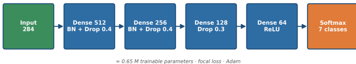
Figure 6. Proposed optimized deep neural network (284 inputs, four hidden layers, 7-way softmax output).
