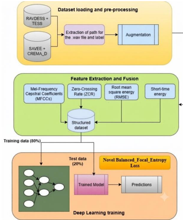
Figure 2. Dataset loading, pre-processing, feature extraction and deep-learning training pipeline.
