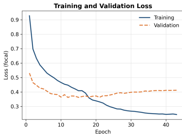
Figure 8. Training and validation loss across epochs.
