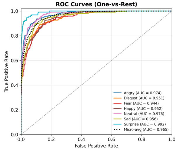
Figure 10. Per-class ROC curves with areas under the curve on the combined test set.
