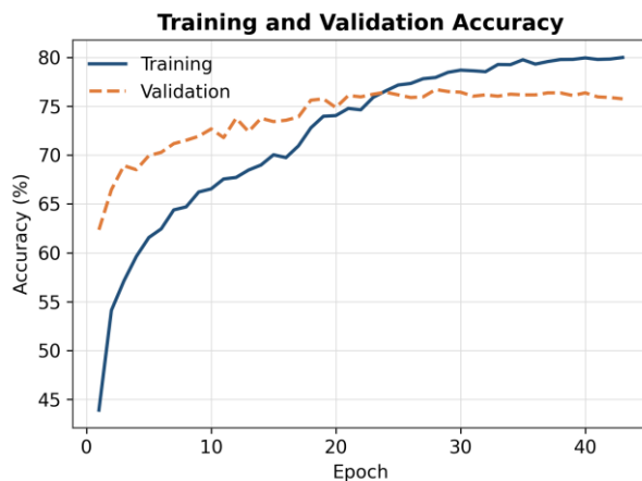
Figure 7. Training and validation accuracy across epochs.
