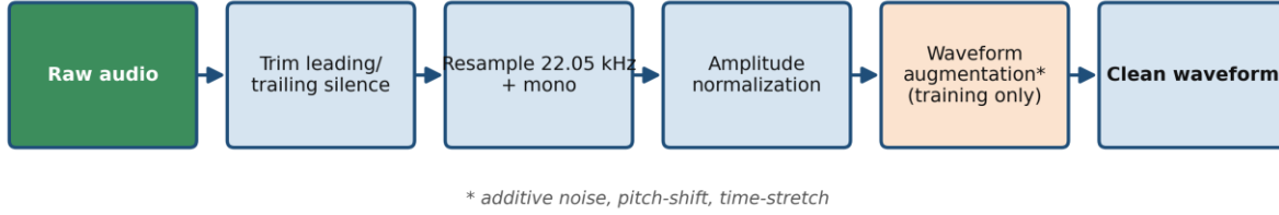
Figure 3. Audio preprocessing workflow applied uniformly to uploaded and recorded audio.
