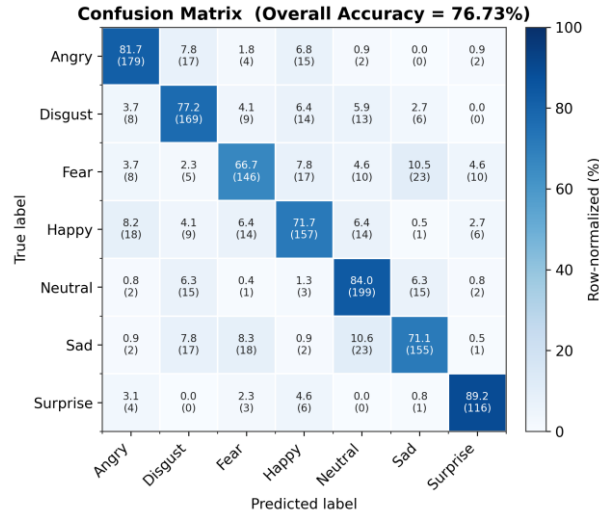
Figure 9. Row-normalized confusion matrix on the combined test set (percentages; counts in parentheses).
