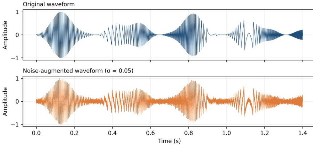
Figure 4. Illustration of additive-noise augmentation: an original waveform (top) and its augmented version (bottom).
